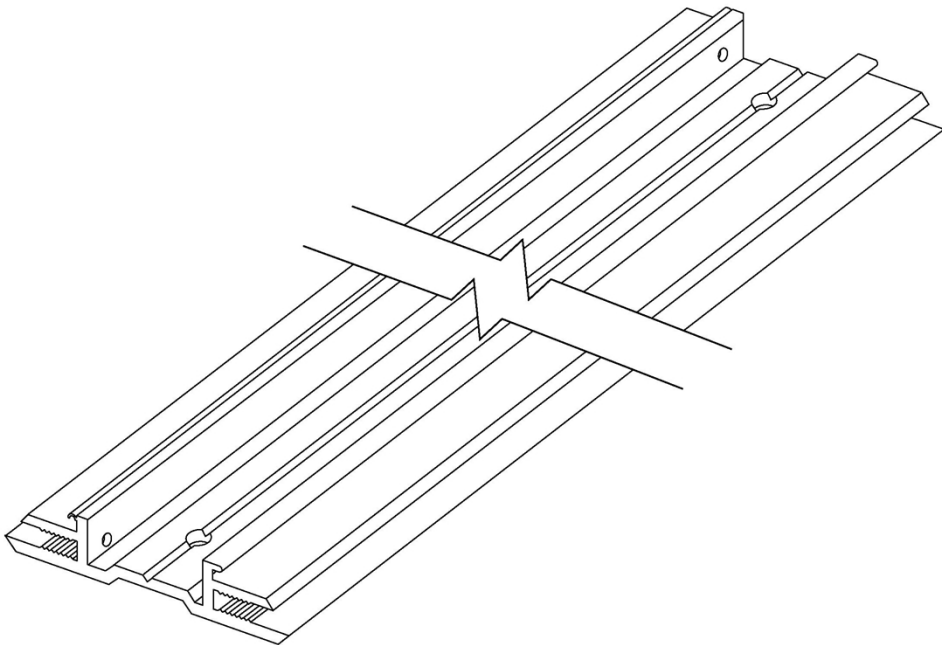
ISOMETRIC VIEW WITHOUT COVER
