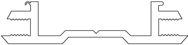
TOP VIEW WITHOUT COVER
